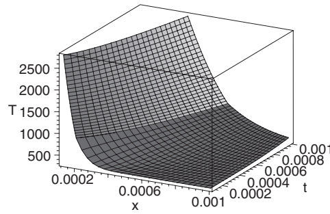
Figure 1. Exact solution of problem (1)–(7) with parameters that are typical for aluminium: \lambda_1 = \lambda_2 = 240 \text{ W K}^{-1} \text{ m}^{-1} , C_1 = 2.7 \times 10^6 \text{ J K}^{-1} \text{ m}^{-3} , C_2 = 2.74 \times 10^6 \text{ J K}^{-1} \text{ m}^{-3} , H_v = 2.69 \times 10^{10} \text{ J m}^{-3} , H_m = 0.17 \times 10^{10} \text{ J m}^{-3} , T_0 = 300 \text{ K} , T_m = 933 \text{ K} and T_v = 2793 \text{ K} ; the energy flux was set q = \frac{2.5 \times 10^8}{\sqrt{t}} \text{ W m}^{-2} .
